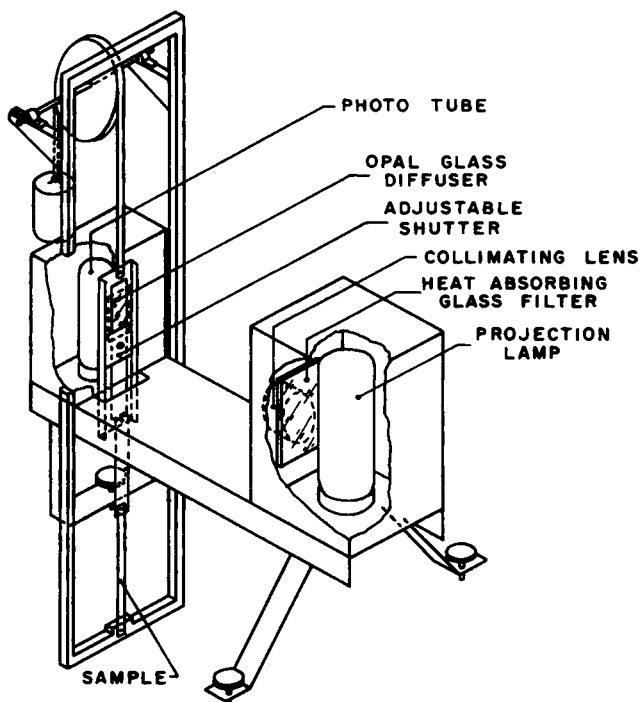
Fig. 1. Assembled components.
