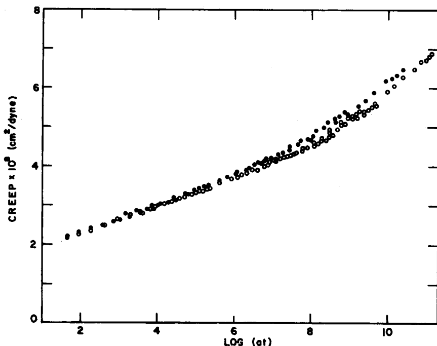
Fig. 4. Creep data reduced to 41°C.: (O) recorder; (●) cathetometer.
