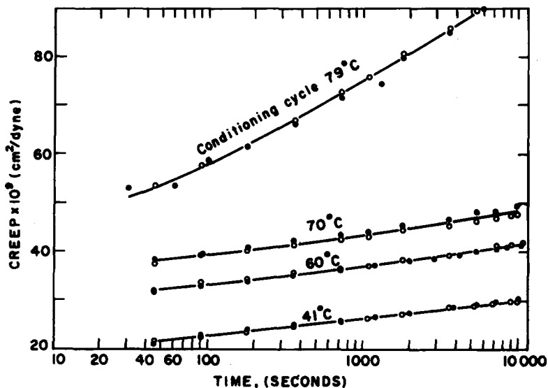
Fig. 3. Creep curves at various temperatures, comparing data obtained with the recorder and the cathetometer: (O) recorder; (●) cathetometer.
