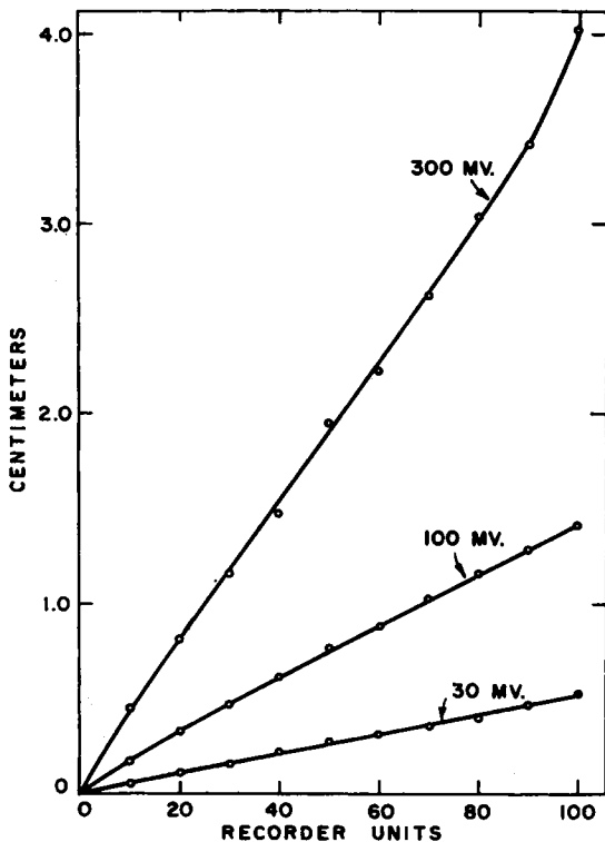
Fig. 2. Calibration graph.
